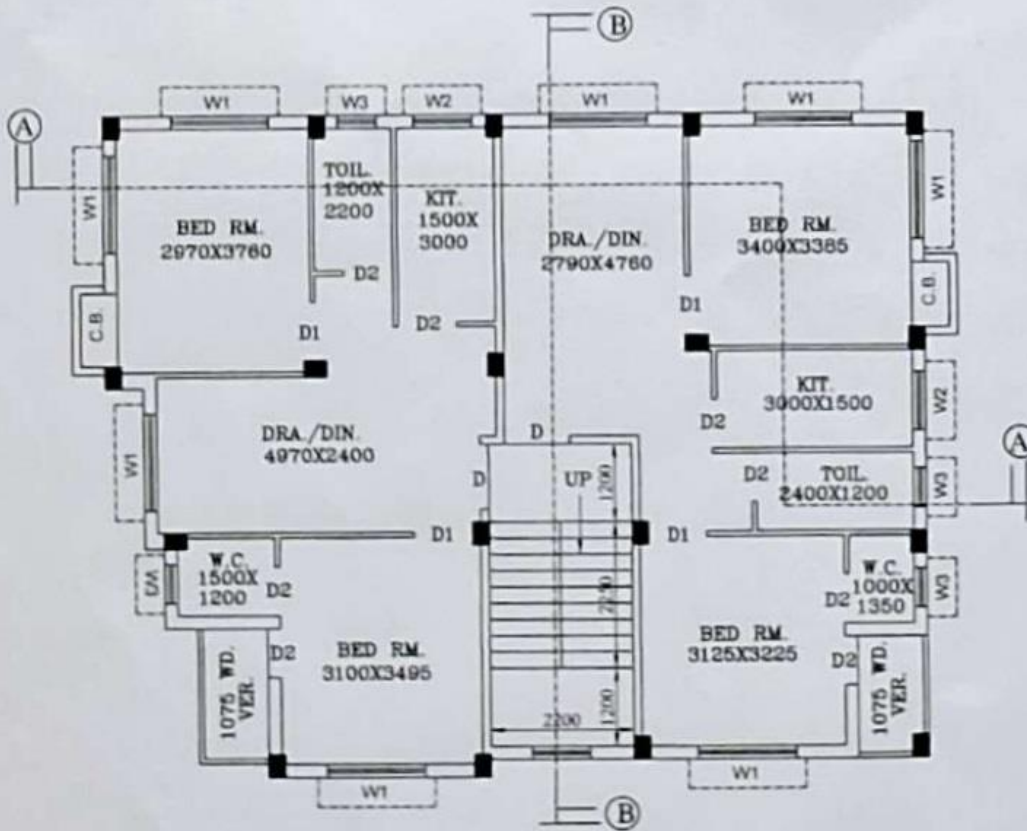
FIRST & SECOND FLOOR PLAN SCALE :-1:100
